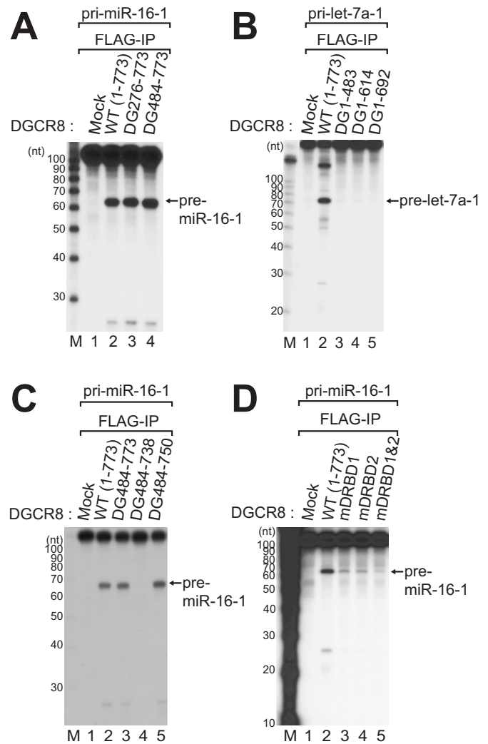
Figure 4. DGCR8 domains required for pri-miRNA processing. In vitro pri-miRNA processing assay of DGCR8 mutants. FLAG-DGCR8 was immunoprecipitated using anti-FLAG antibody-conjugated agarose beads in low salt buffer (buffer D-K'200), and subsequently subjected to an in vitro pri-miRNA processing assay. Pri-miR-16-1 or pri-let-7a-1, labeled internally with 32 P-UTP, was used as the substrate. Decade markers (Ambion) were used as the size markers.
