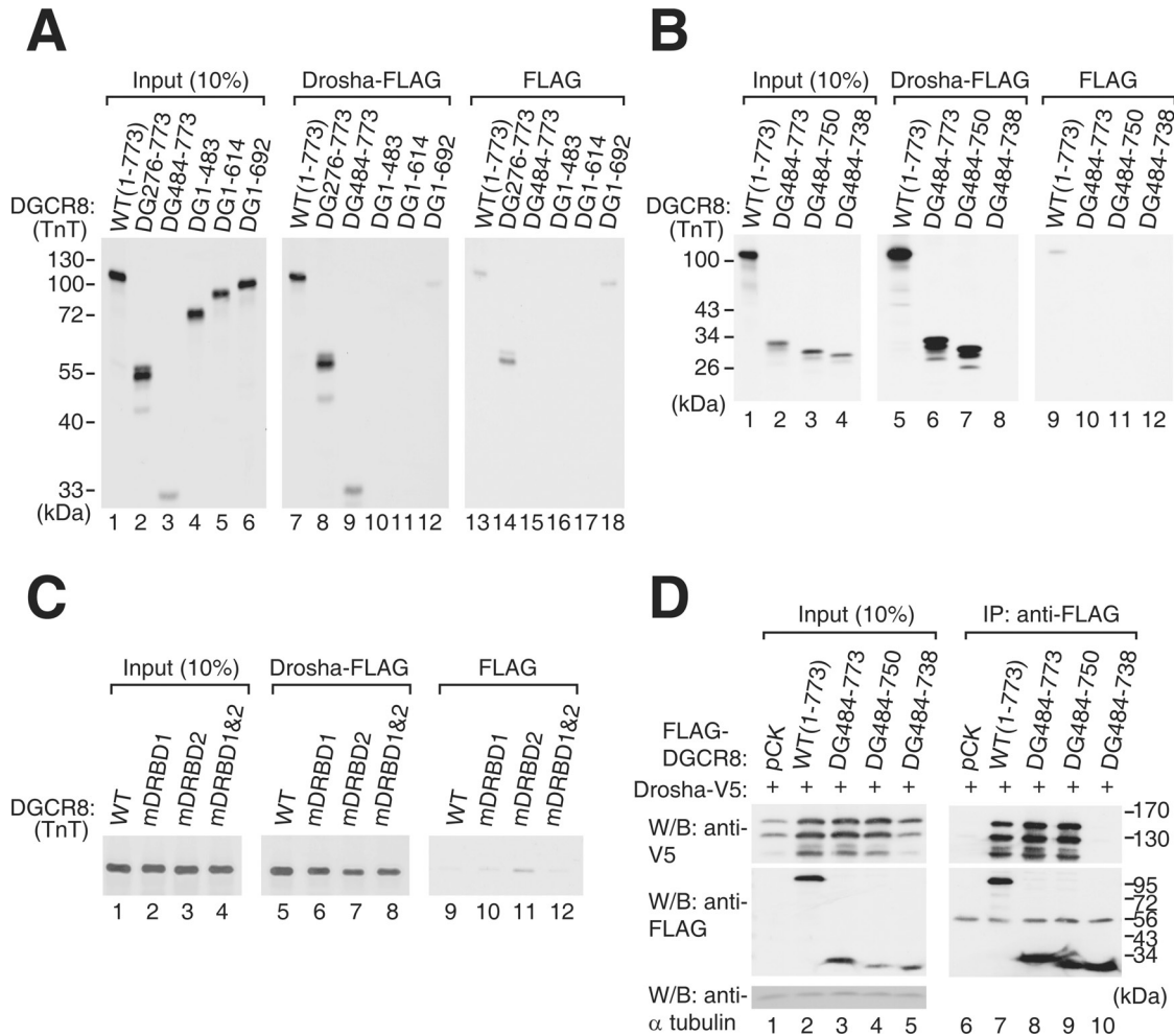
Figure 2. Identification of the Drosha-interacting domain. (A–C) In vitro binding assay. DGCR8 wild-type and the indicated mutant proteins were synthesized by TnT ( in vitro transcription and translation, Invitrogen) reactions and incubated with the Drosha-FLAG protein immobilized on anti-FLAG antibody that is conjugated on agarose beads. The left panels show 10% of the input proteins used in the binding reactions, whereas the middle panels visualize the proteins interacting with Drosha-FLAG. As a control (right panels, pull-down with FLAG), an empty vector expressing FLAG tag only was transfected and the cell lysates were used for immunoprecipitation. (D) Immunoprecipitation followed by western blot analysis. FLAG-DGCR8 mutant constructs were co-expressed with Drosha-V5. Immunoprecipitation was performed with anti-FLAG antibody and western blotting was carried out using either anti-V5 antibody (upper panels) or anti-FLAG antibody (lower panels).
