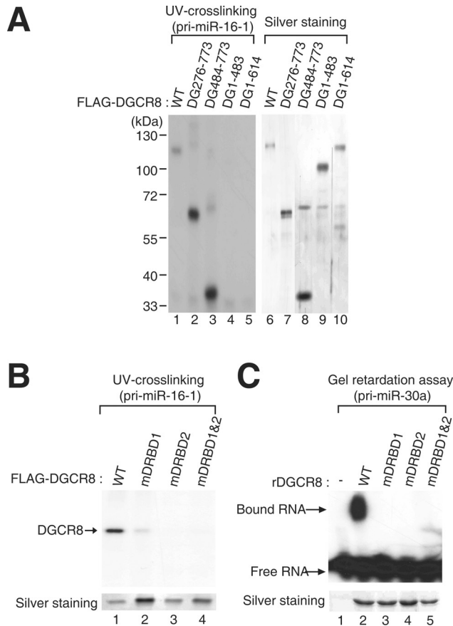
Figure 3. DGCR8 domains responsible for pri-miRNA binding. (A) UV-crosslinking experiments between a series of DGCR8 deletion mutants and 32 P-UTP radiolabeled pri-miR-16-1. After UV-crosslinking, residual RNA was removed by treatment with an RNase A/T1 mix. The left panel visualizes the radioactivity associated with recombinant FLAG-DGCR8 proteins, whereas the right panel indicates the amounts of protein used in this experiment as visualized by silver staining. (B) UV-crosslinking between a series of DGCR8 point mutants and 32 P-UTP radiolabeled pri-miR-16-1. The upper panel displays the radioactivity crosslinked to the immunopurified FLAG-DGCR8 proteins and the lower panel indicates the amount of protein used in this experiment as determined by silver staining. (C) Gel retardation assay of pri-miR-30a binding to DGCR8 point mutants. Recombinant DGCR8 proteins prepared from E.coli were pre-treated with thrombin to separate the GST tag prior to the assay. The lower panel shows silver stained gel of recombinant DGCR8 protein used in this experiment.
